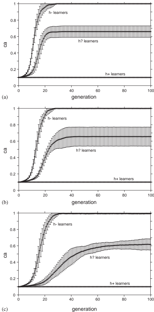
Fig. 1. Cultural evolution as a consequence of learner biases, with various levels of noise. (a) gives results for \rho = 0 , (b) gives results for \rho = 0.05 , (c) gives results for \rho = 0.1 .
