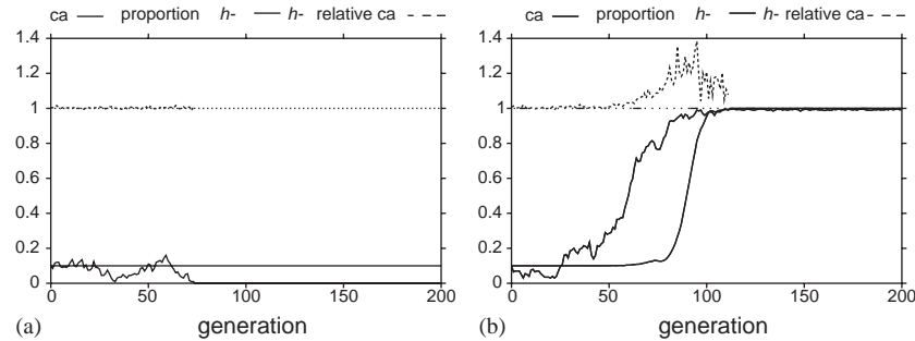
Fig. 3. The evolution of learning biases in a majority h+ population converged on a fully homonymous system. (a) shows a run where drift eliminates h- learners before the cultural construction process gets underway. (b) shows a run where drift preserves h- learners in sufficient numbers for their learning bias to take effect. They are then selected for, and the population converges on an optimal vocabulary system.
