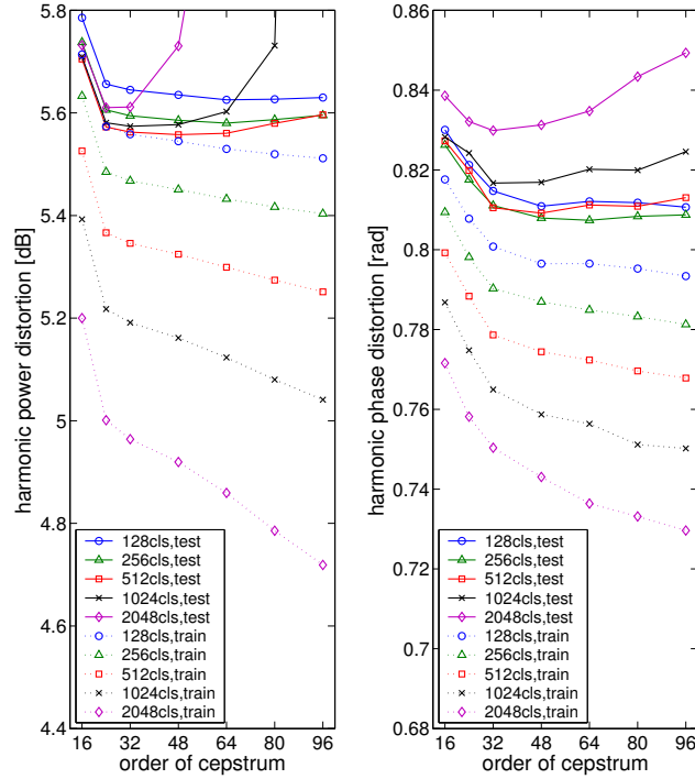
Figure 6: Harmonic distortion vs. order of cepstrum, in the case of the piecewise constant mapping
