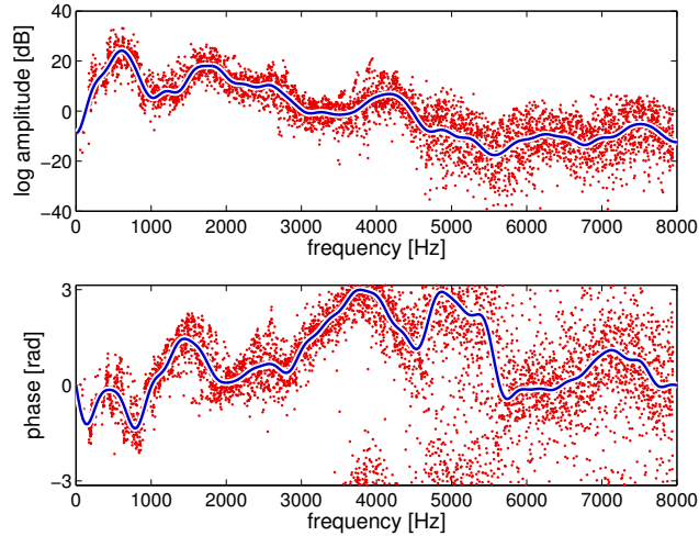
Figure 5: Spectral envelopes of one of the articulatory clusters computed using the piecewise constant approximation
