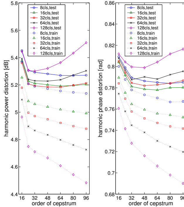
Figure 7: Harmonic distortion vs. order of cepstrum, in the case of the piecewise linear mapping
