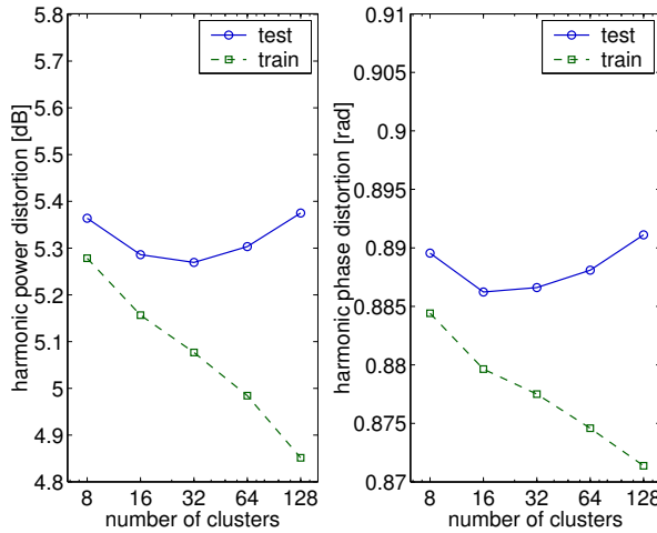
Figure 3: Harmonic distortion vs. number of clusters, based on cepstral domain criteria for the piecewise linear mapping
