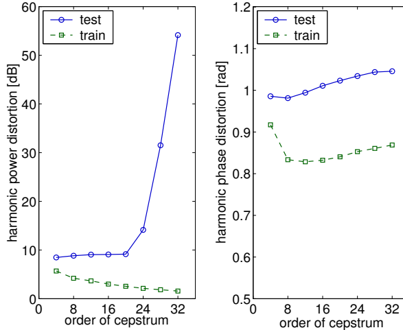
Figure 1: Harmonic distortion vs. order of cepstrum, when each cluster comprises only one frame
