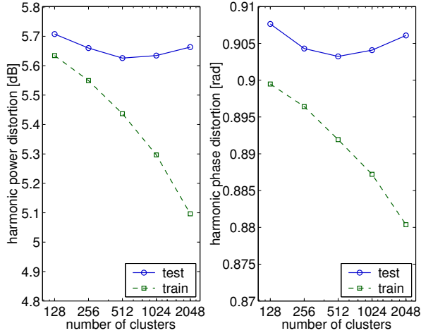
Figure 2: Harmonic distortion vs. number of clusters, based on cepstral domain criteria for the piecewise constant mapping
